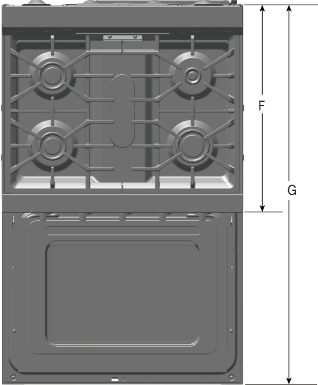
TOP VIEW
