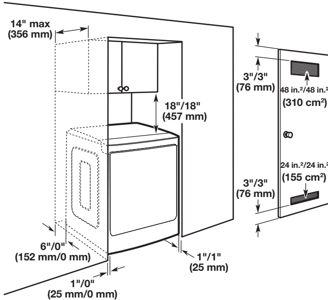
Recommended/Minimum spacing
