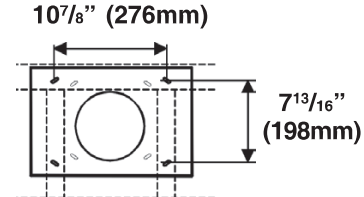
TOP VIEW OF SUPPORT FRAME
