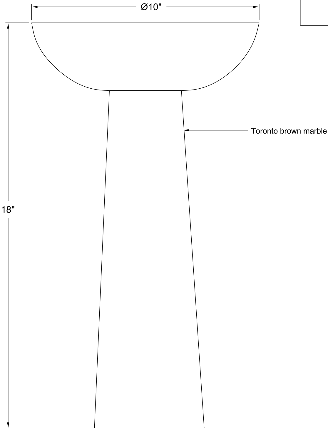
FRONT VIEW
