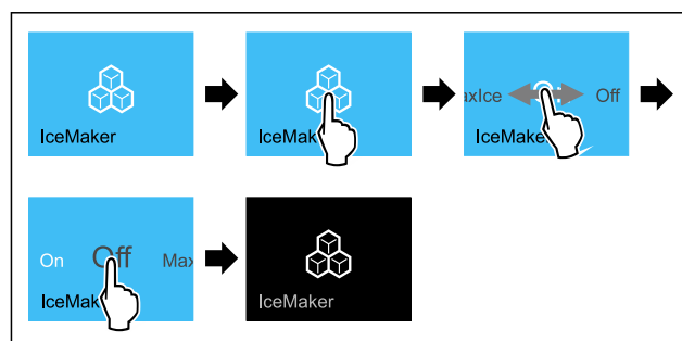
Fig. 77 Example illustration of the active IceMaker function
