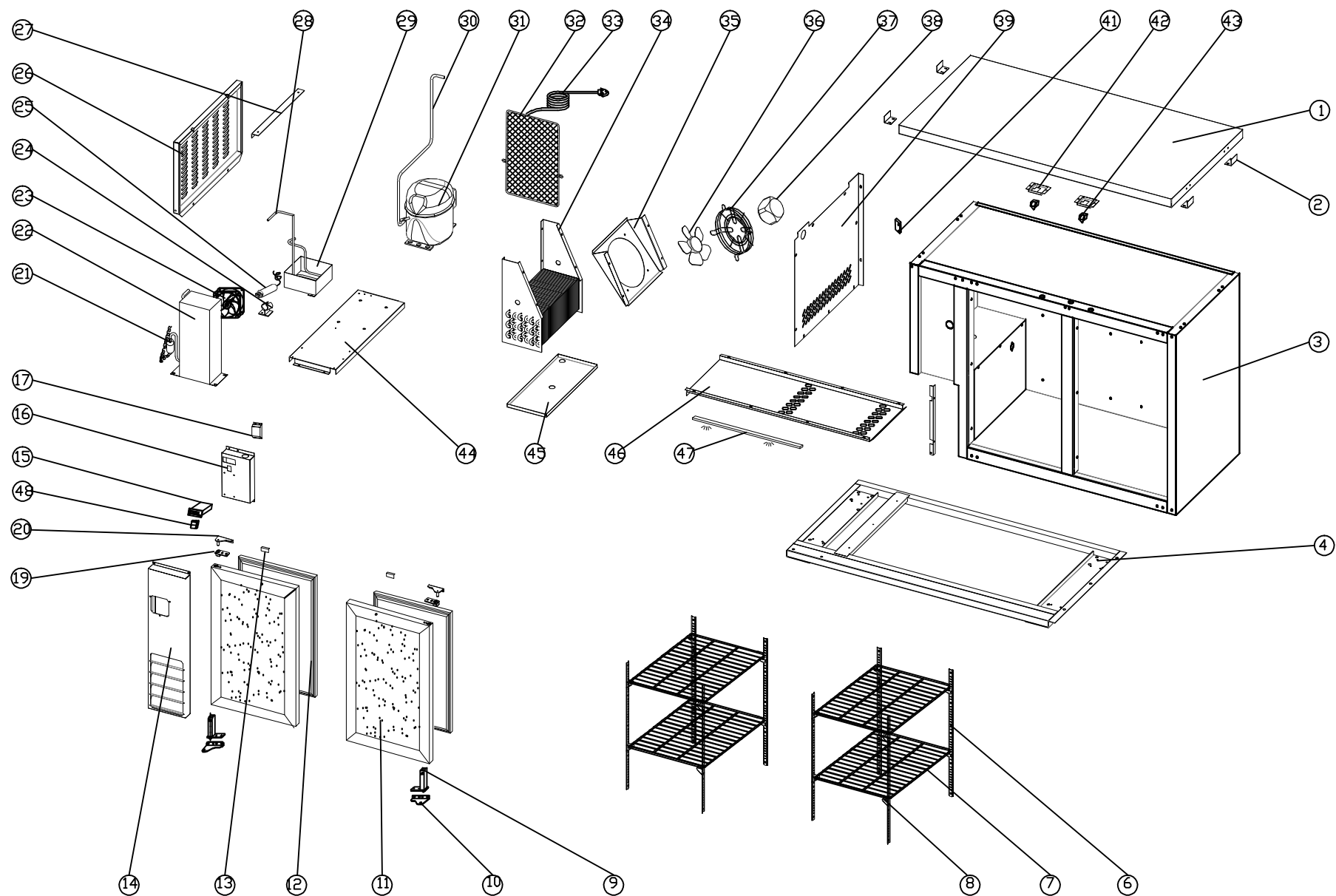
KELVINATOR COMMERCIAL KCHBB48G - exploded view
