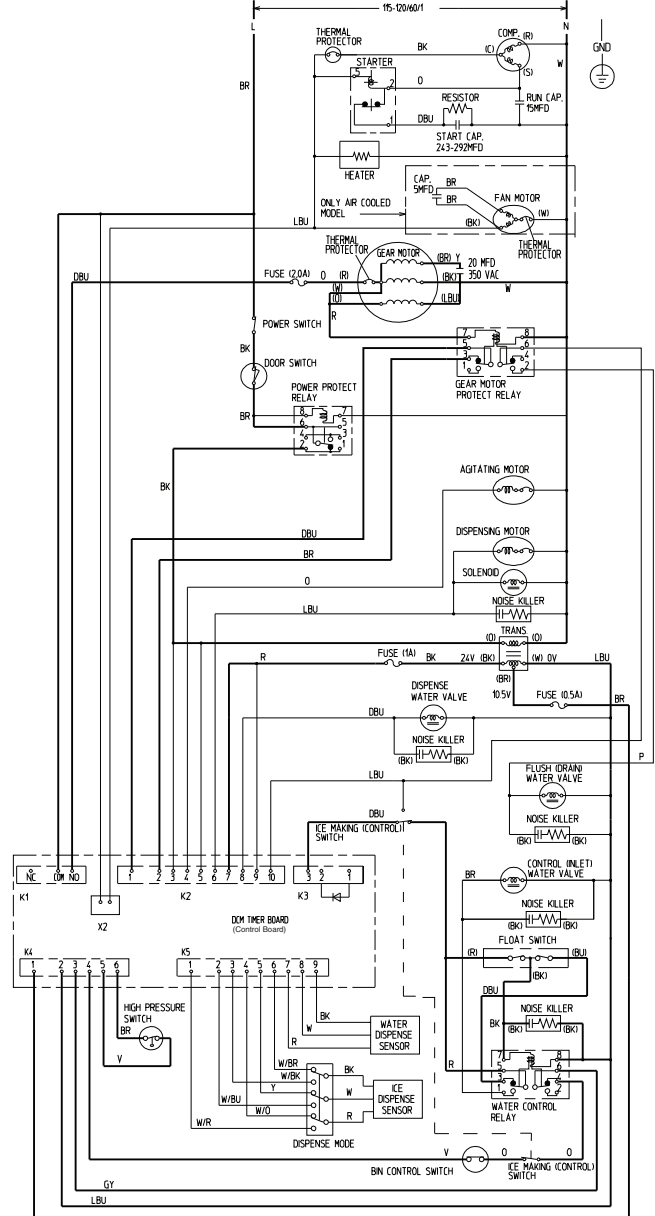
DCM-500BAH-OS DCM-500BWH-OS WIRING DIAGRAM
