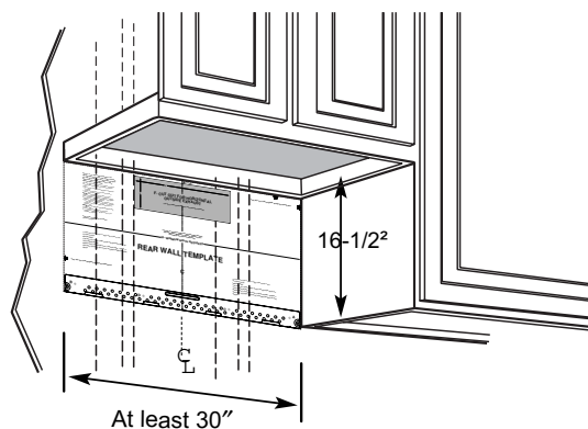
Plate position—beneath flat bottom cabinet
