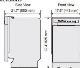
Product dimensions
