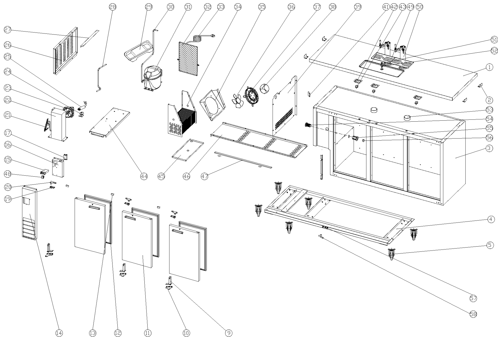
KELVINATOR COMMERCIAL - KCHBBD3D2T exploded view
