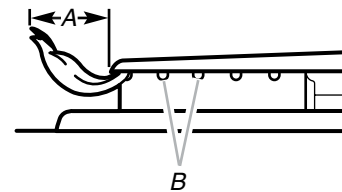
A. 1 to 1½" (2.5 to 3.8 cm) B. Burner ports
