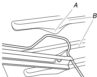
A. “V” cutout B. Rack guides
