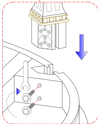
detail 'A'
