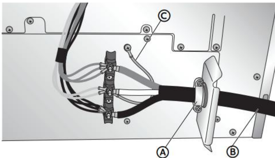
A UL Listed Strain Relief
