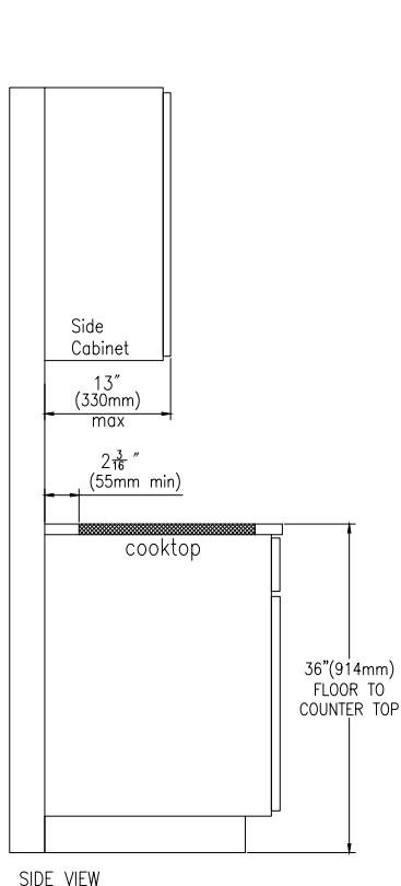
SIDE VIEW
