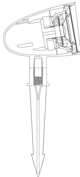
Satellite Speaker Side View
