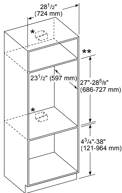
Single Oven Wall Mount Installation
