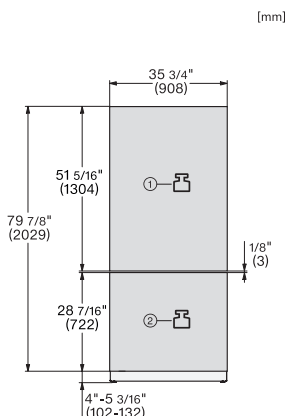
KFMC3642R, KFMC3842L, KFMC3844R, KFMC3844L, MasterCool III, front view
