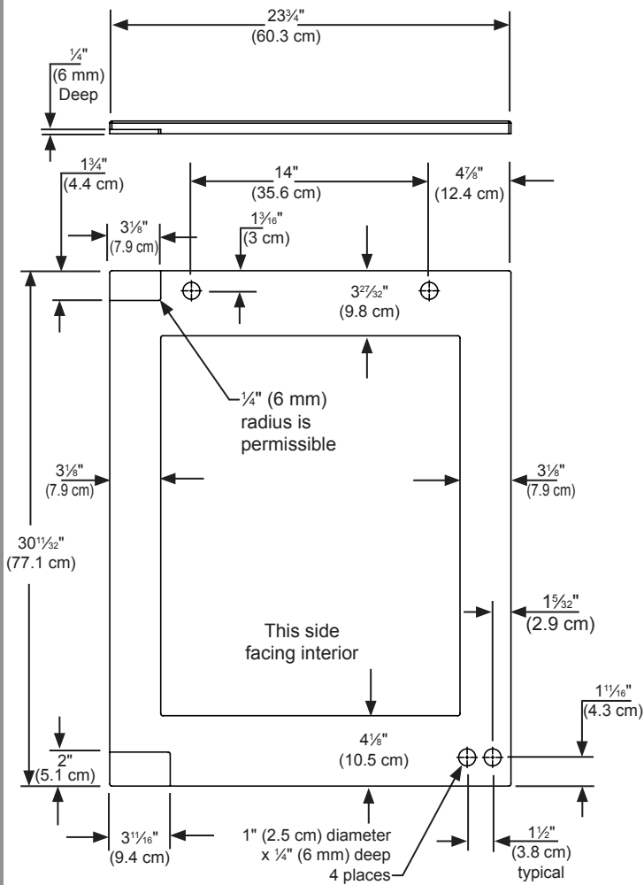
Figure 18 Right Hand Hinged Door 24" (61 cm) wide appliance
