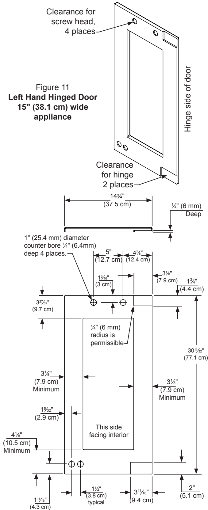
Figure 12 Left Hand Hinged Door 15" (38.1 cm) Wide Appliance
