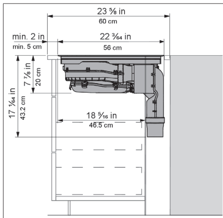
Fig. 1.2 Recirculation Kit sample planning
