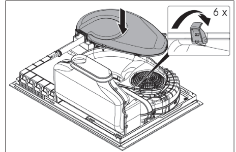
Fig. 1.7 Mounting the air guide housing
