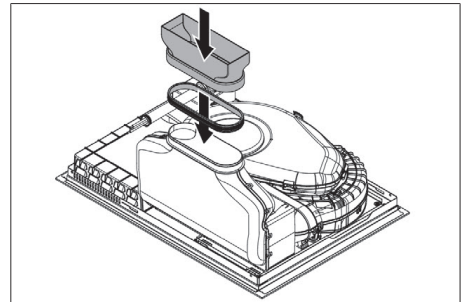
Fig. 1.8 Mounting the exhaust air adapter
