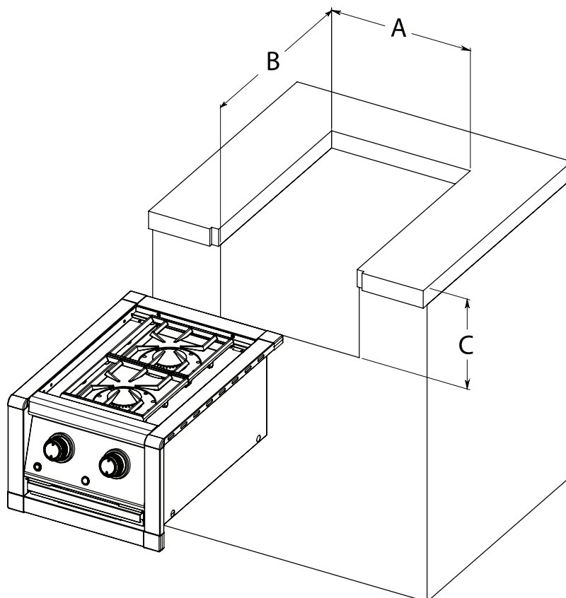
BROIL KING® IMPERIAL™ S 200 RANGE BURNER
