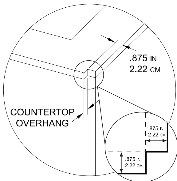
COUNTER TOP NOTCH DETAIL
