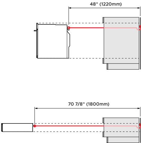
PROFILE VIEW
