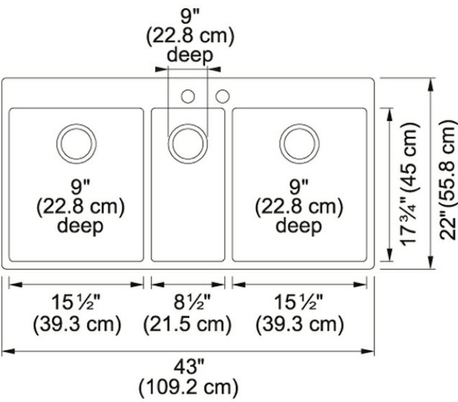
Technical Drawing
