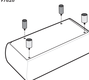
12.5 cm/4.92 inch Ø 4.2 cm 2x 1997826
