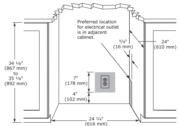
Cabinet Cut-Out
