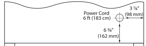
Cabinet Cut-Out
