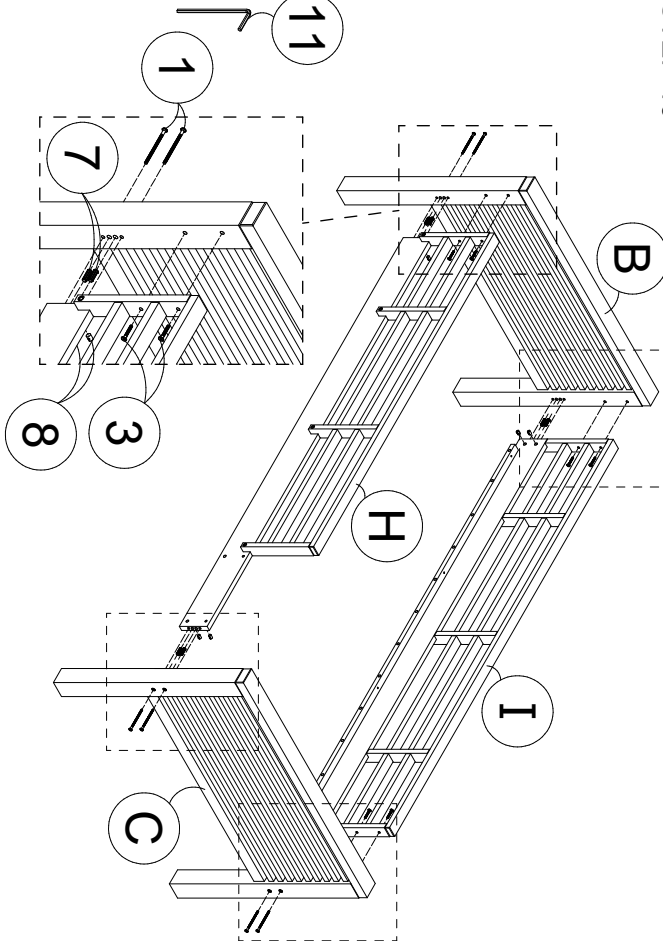
STEP 10
