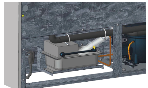
Install heated condensate pan and place drain pipe in pan*
