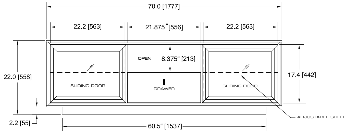
FRONT VIEW
