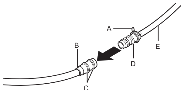
A. Small clamp B. Rubber drain hose connector C. Stop D. Drain hose stop E. Drain hose
