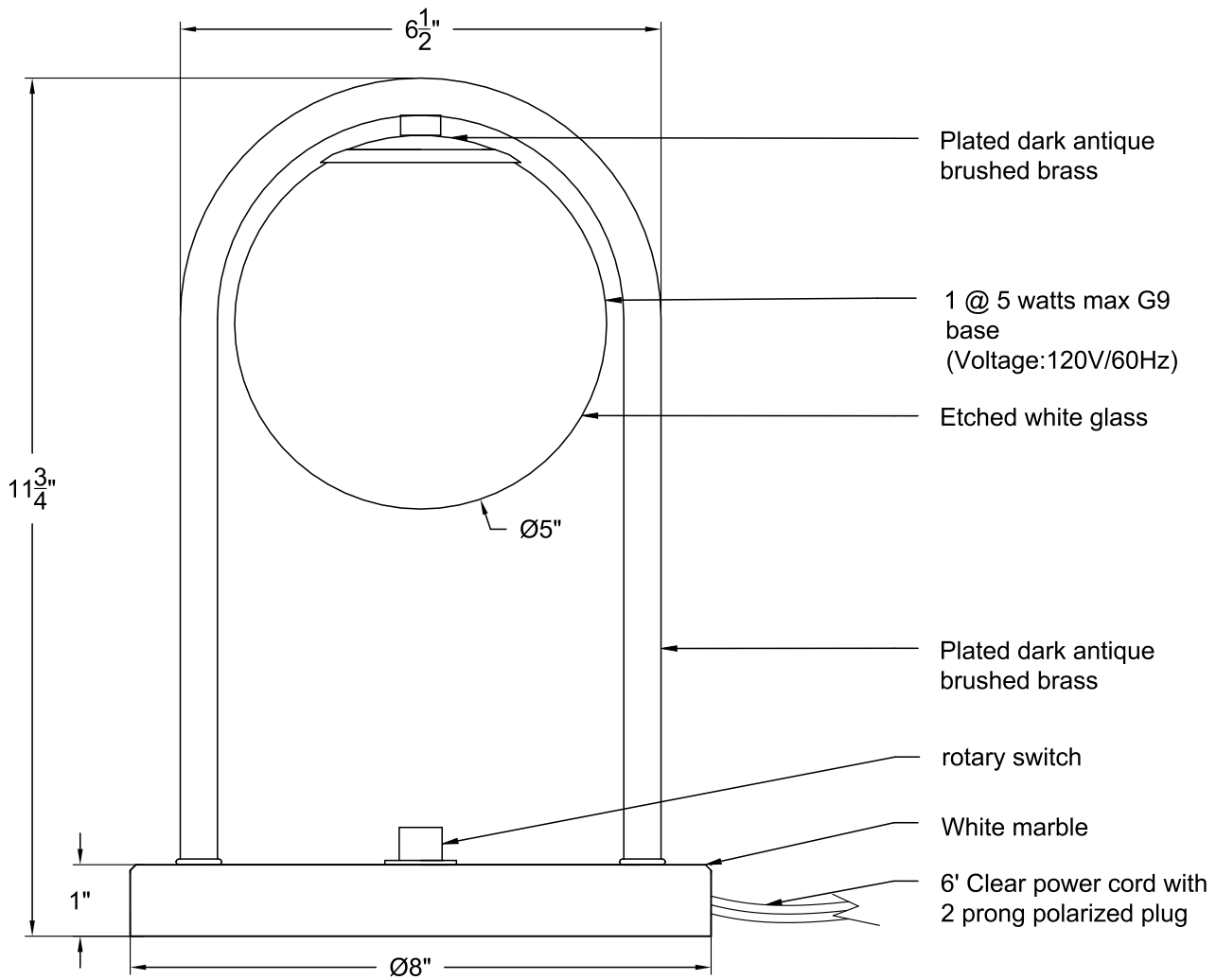
FRONT VIEW
