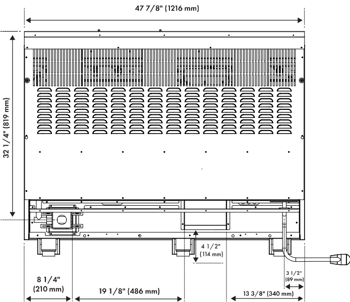
BACK VIEW
