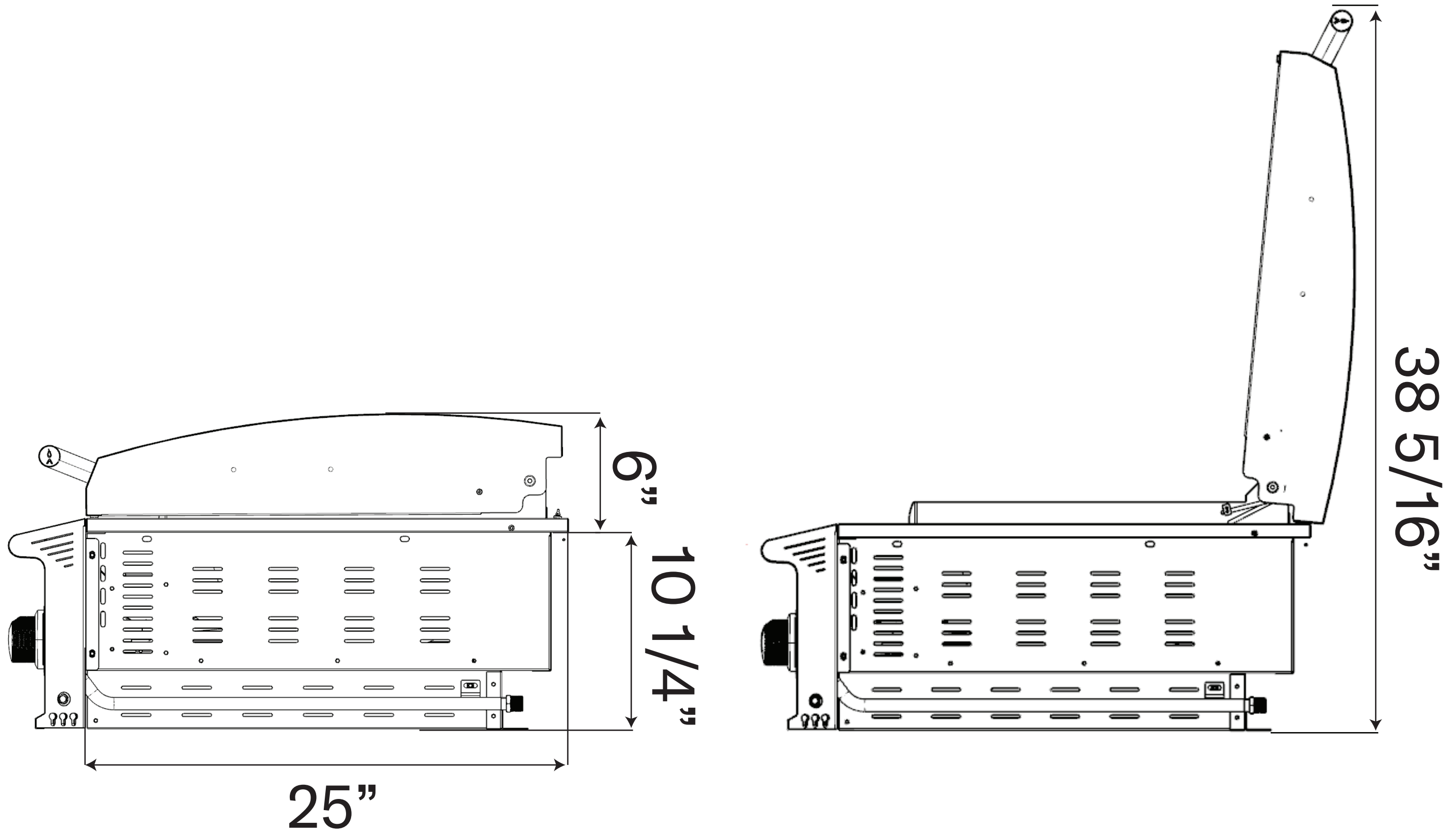
Side View
