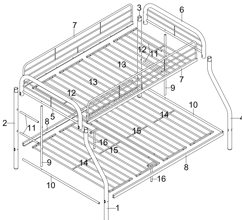
Exploded View
