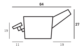
Side View (standard mechanism, fully reclined)
