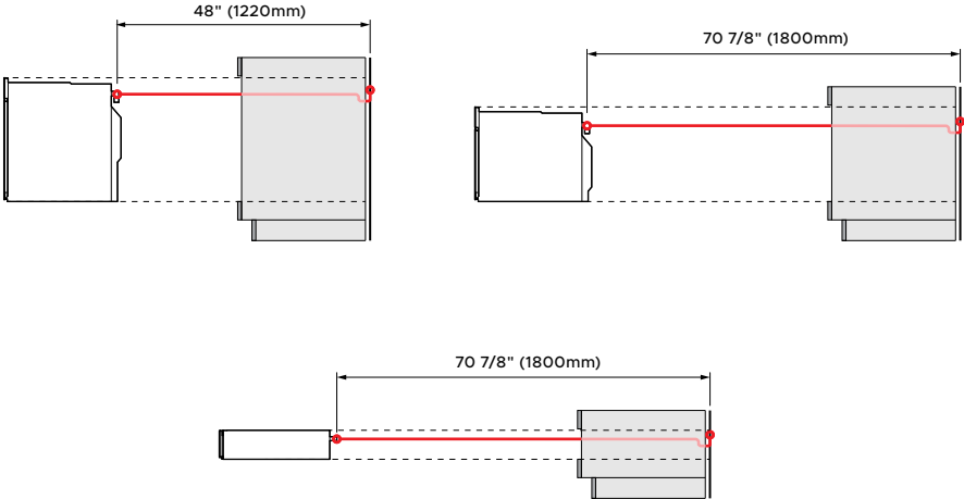
PROFILE VIEW
