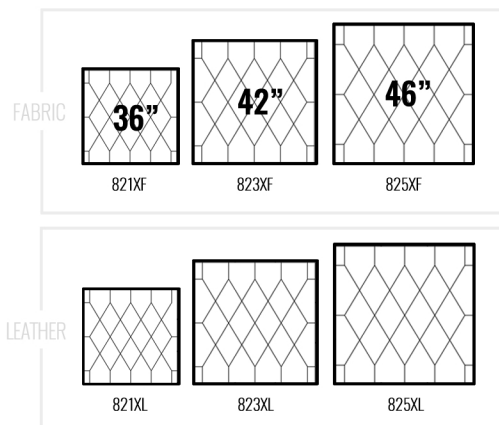
FABRIC / LEATHER SEAM PLACEMENT
