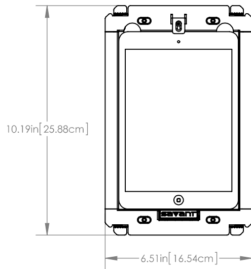
Front View without Bezel
