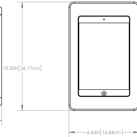
Front View with Bezel
