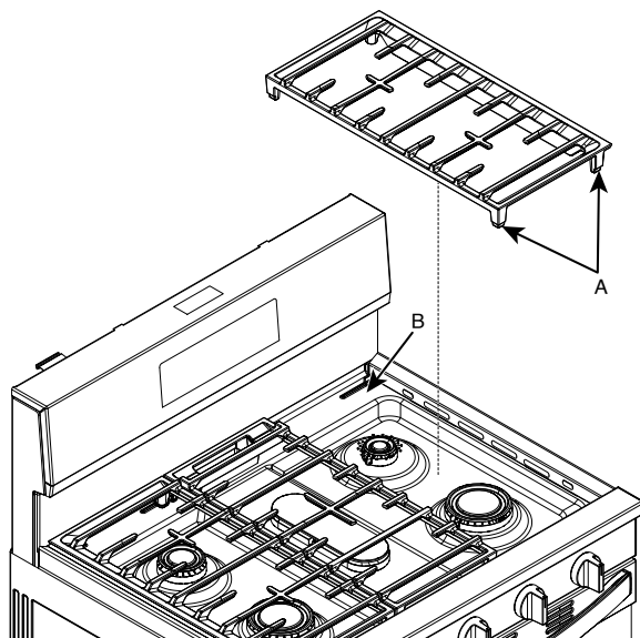
A. Bumpers B. Alignment indentations
