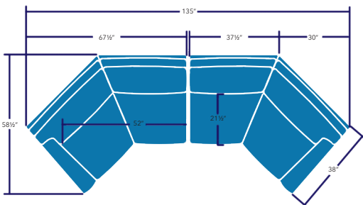
LEFT/RIGHT ARM FACING WEDGE LOVESEAT 47 - 2/2 - LW/RW OVERALL: H36 W67½ D58½ INSIDE: W52 D21½ SEAT: H20 ARM: H25½
