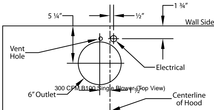
CONNECTION DIAGRAM
