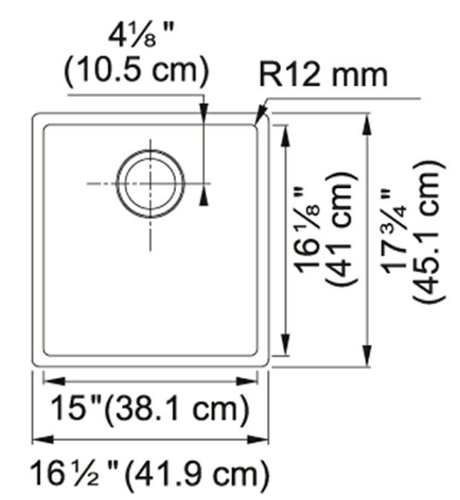
Technical Drawing
