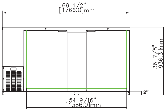
BB69(-S) Front View
