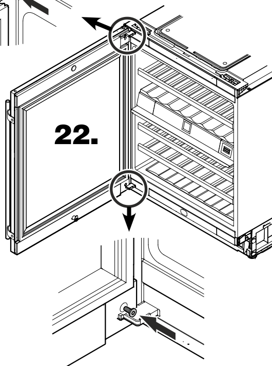
22. Screw in the screws at the top and bottom.
