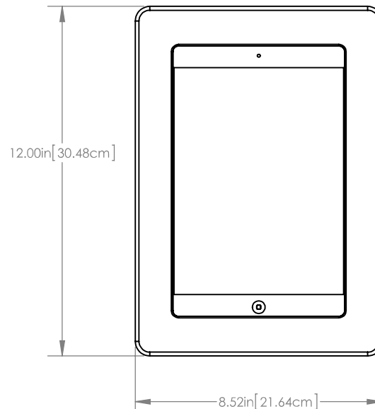
Front View with Bezel
