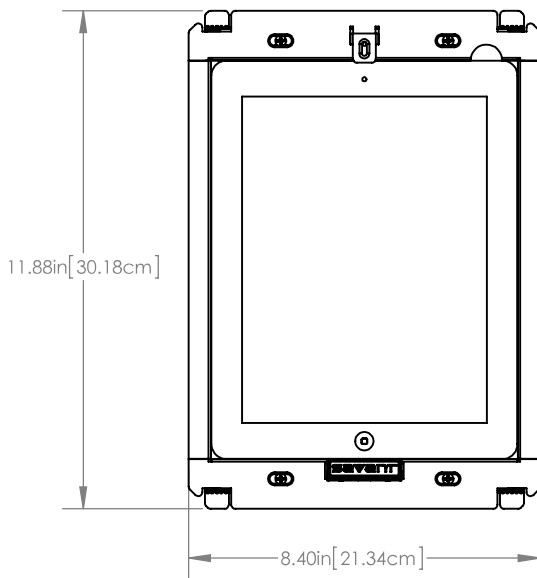
Front View without Bezel
