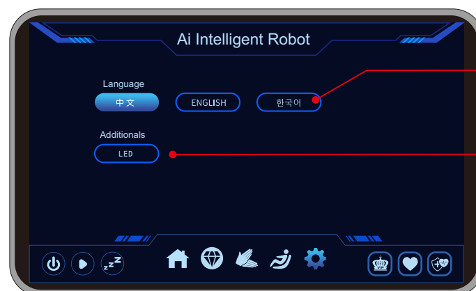
Settings Interface
