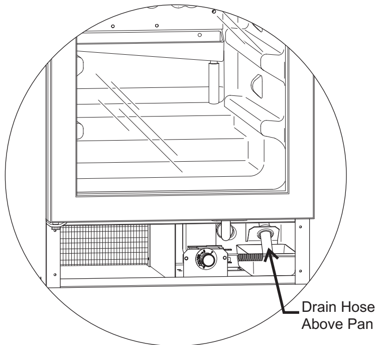
Detail of Drain System
