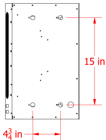
TOP VIEW (CLOSED)
