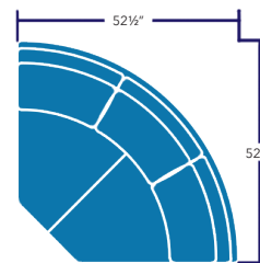
ROUND CHAIR 111 - 3/1 - R OVERALL: H36½ W73 D37½ INSIDE: W48½ D25 SEAT: H20½
