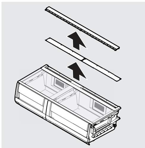
Removing Auto Humidity Control Membrane
