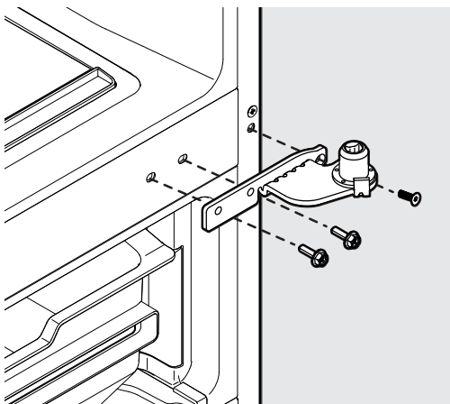
Lower Hinge Removal
