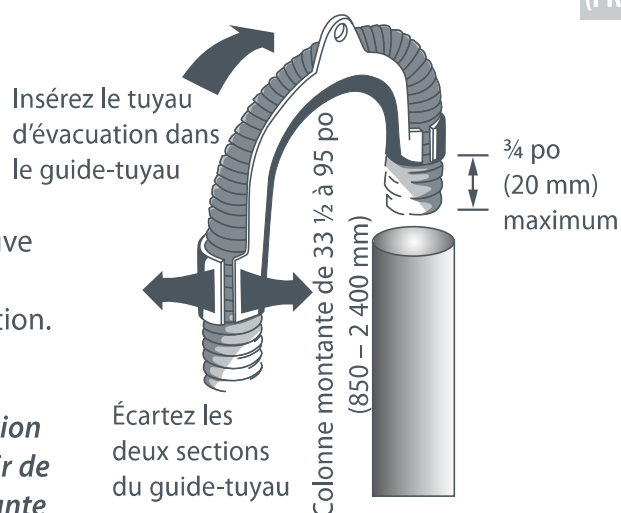
Fig.3 Installation du guide-tuyau
