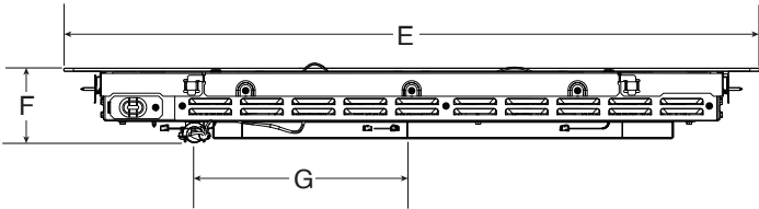
VISTA FRONTAL
